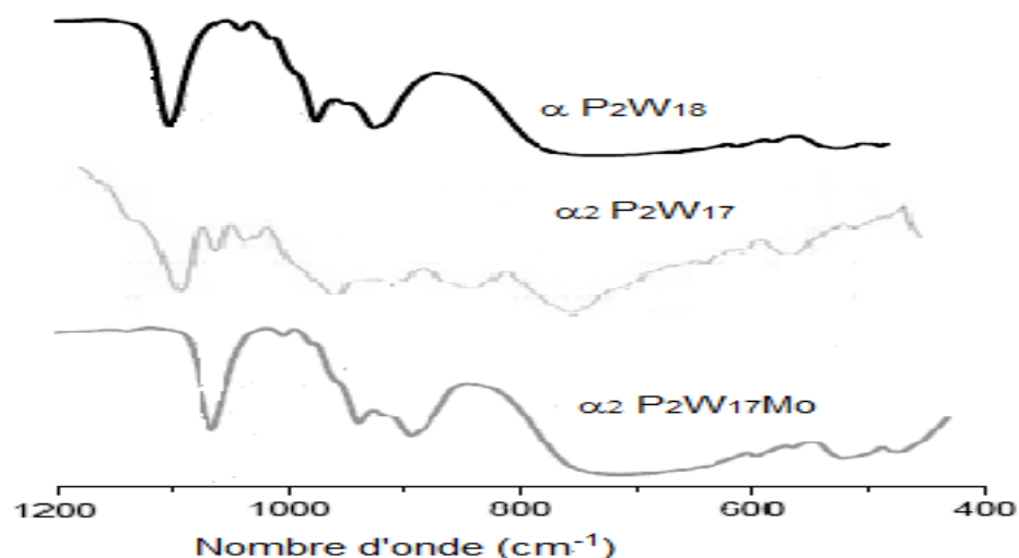
Figure IV-4: Spectre IR du \alpha P 2 W 18 , \alpha_2 P 2 W 17 et \alpha_2 P 2 MoW 17
