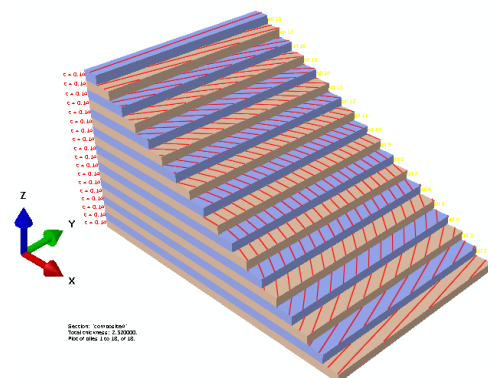
f) Empilement [-80^\circ/-70^\circ/-60^\circ/-50^\circ/-40^\circ/-30^\circ/-20^\circ/-10^\circ/0^\circ/10^\circ/20^\circ/30^\circ/40^\circ/50^\circ/60^\circ/70^\circ/80^\circ/90^\circ]
