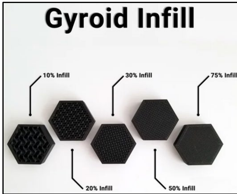
Figure 43. Cut sections with Different % density in gyroid infill pattern.
