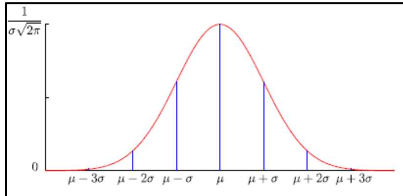
Figure 21. Normal distribution
