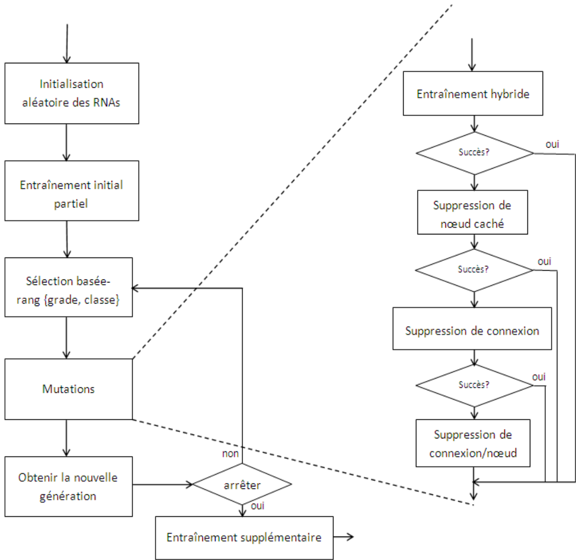
Figure 1.13 : La structure principale d'EPNet [XIN 99]
