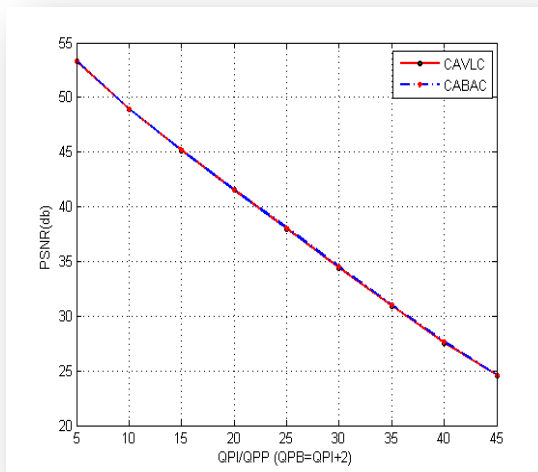
Figure IV.9(a) PSNR Y (CAVLC vs CABAC)
