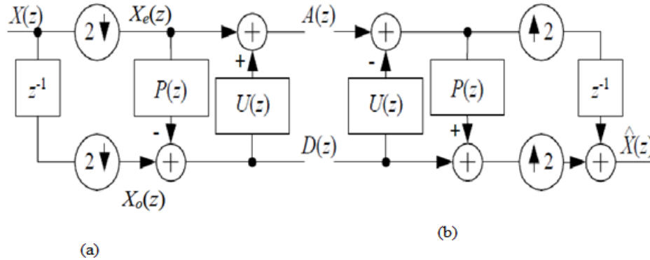
Figure III.8 Lifting scheme. (a) Décomposition, (b) Reconstruction.
