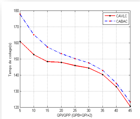
Figure IV.9(c) Temps de codage (CABAC vs CAVLC)
