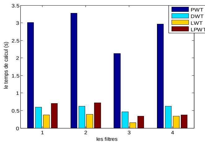
Figure III.9 Comparaison en termes de temps de calcul (image :barbara.png) (1:db5, 2:coif2, 3:sym2, 4:bior2.4) PWT : Packet Wavelet Transform DWT : Discrete Wavelet Transform LWT: Lifting Wavelet Transform LPWT: Lifting Packet Wavelet Transform.
