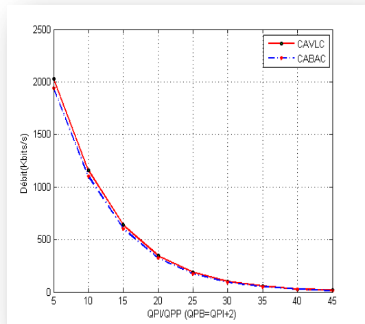
Figure IV.9(b) Débit (CAVLC vs CABAC)
