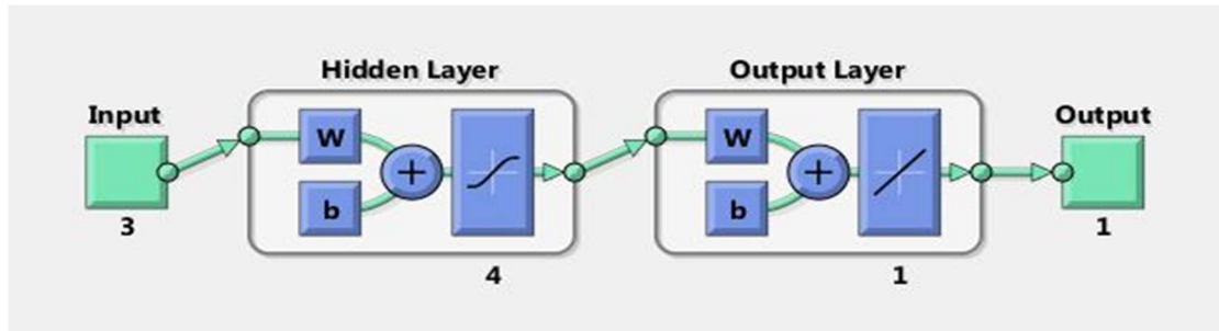
Fig 5.45 Neural network structure of model 4-scenario 1
