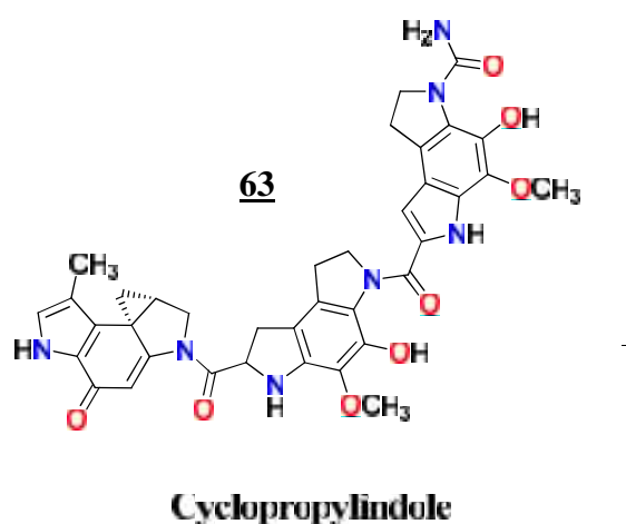
Figure 18 : Structure de la cyclopropylindole.
