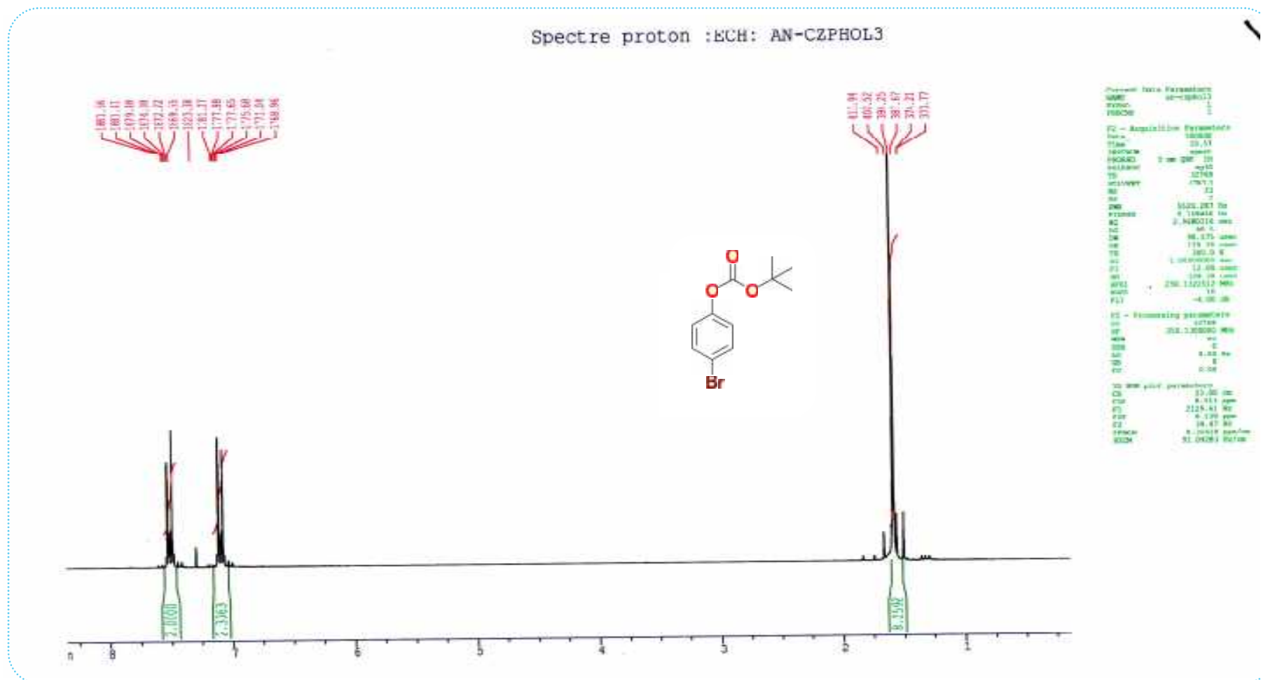
Specter RMN du ^1\text{H} : tert -butyl 4-bromophenyl carbonate
