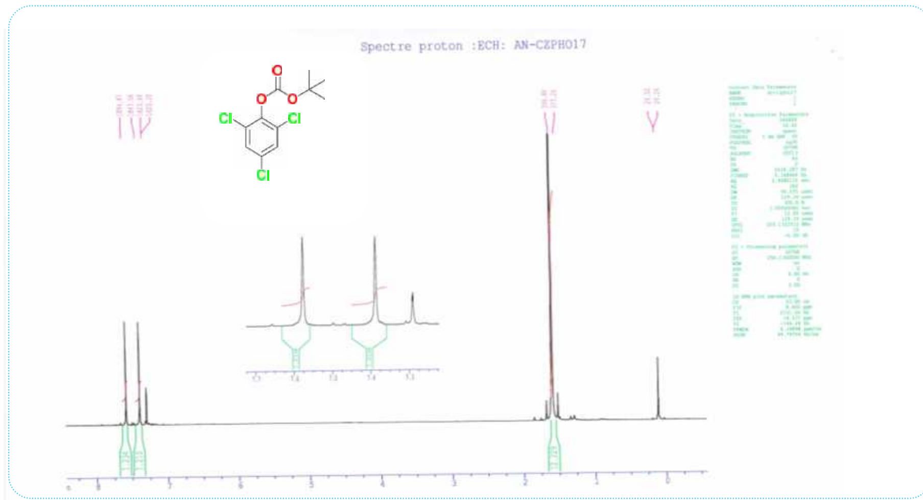
Specter RMN du 1 H: tert-butyl (2,4,6-trichlorophenyl) carbonate
