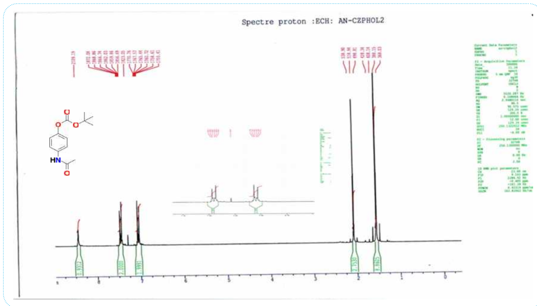
Specter RMN du ^1\text{H} : tert -butyl 4-acetamidophenyl carbonate
